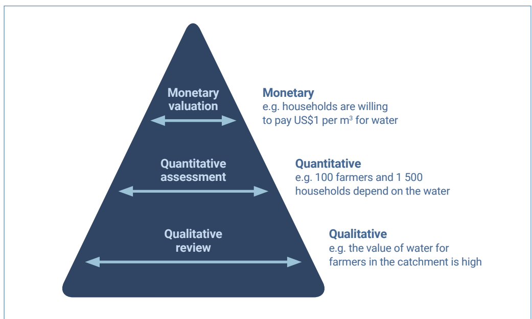
Figure 6.3 Hierarchy of water valuation approaches
