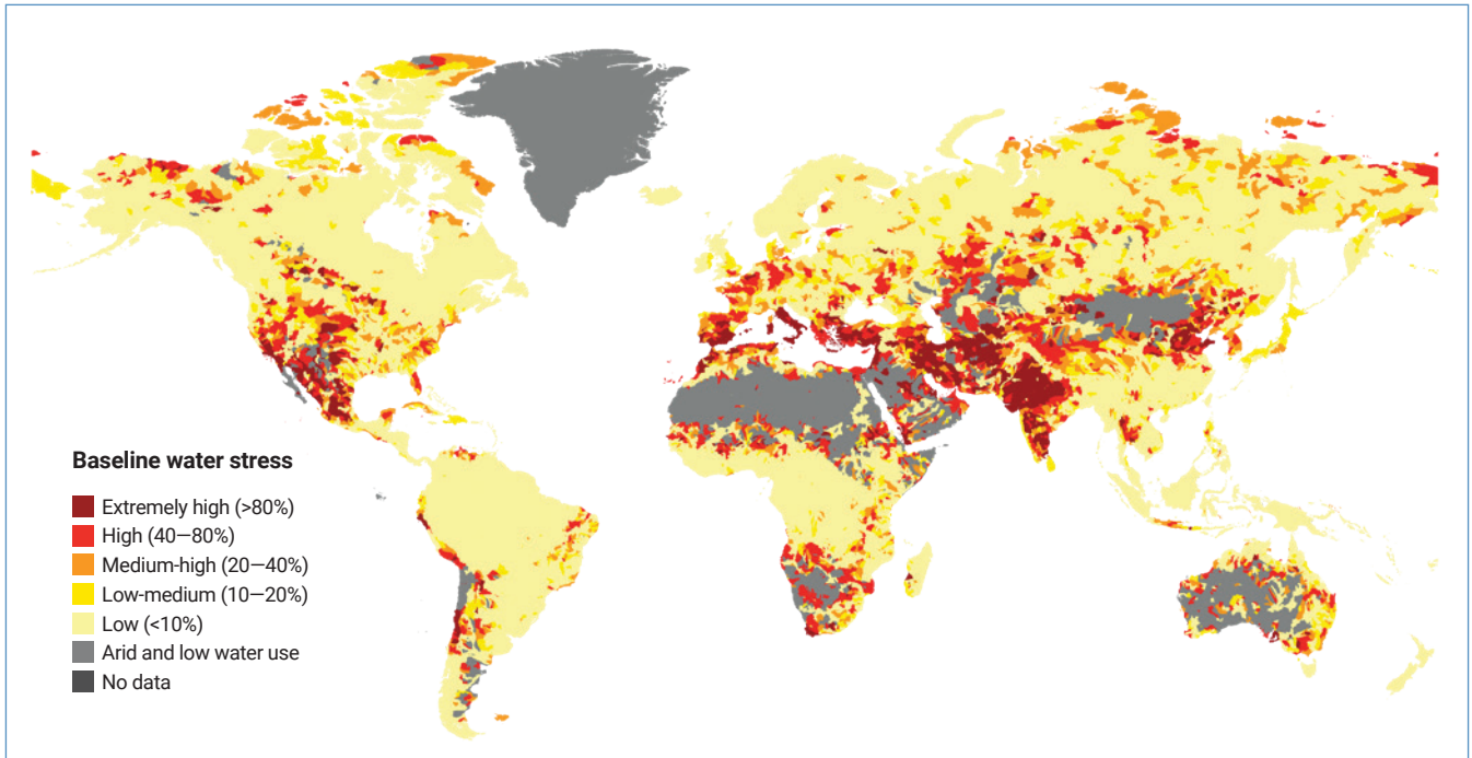
Figure P2 Annual baseline water stress
