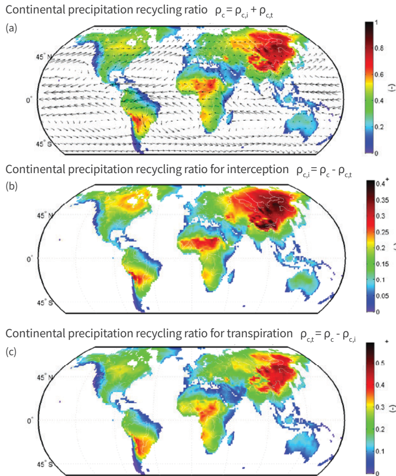
Figure 1.2 Continental precipitation recycling, 1999–2008
