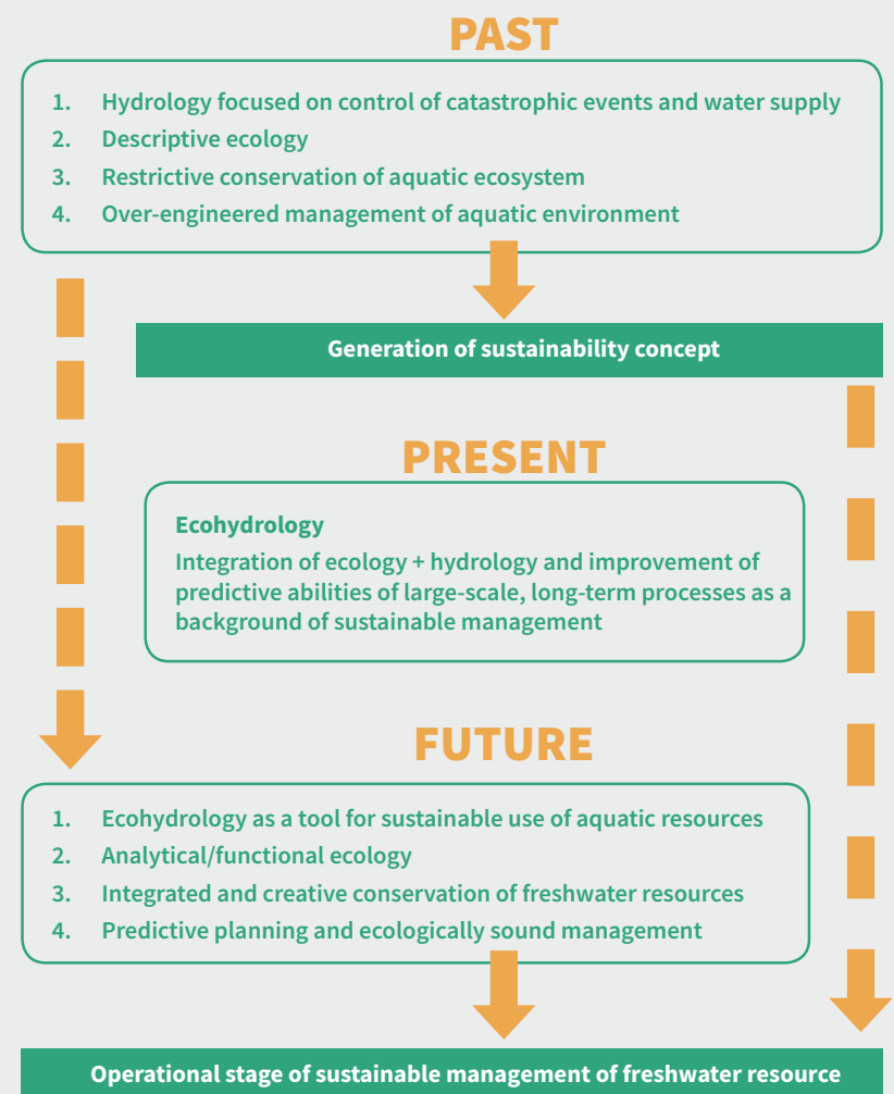
Figure | Ecohydrology: Past, present, future
