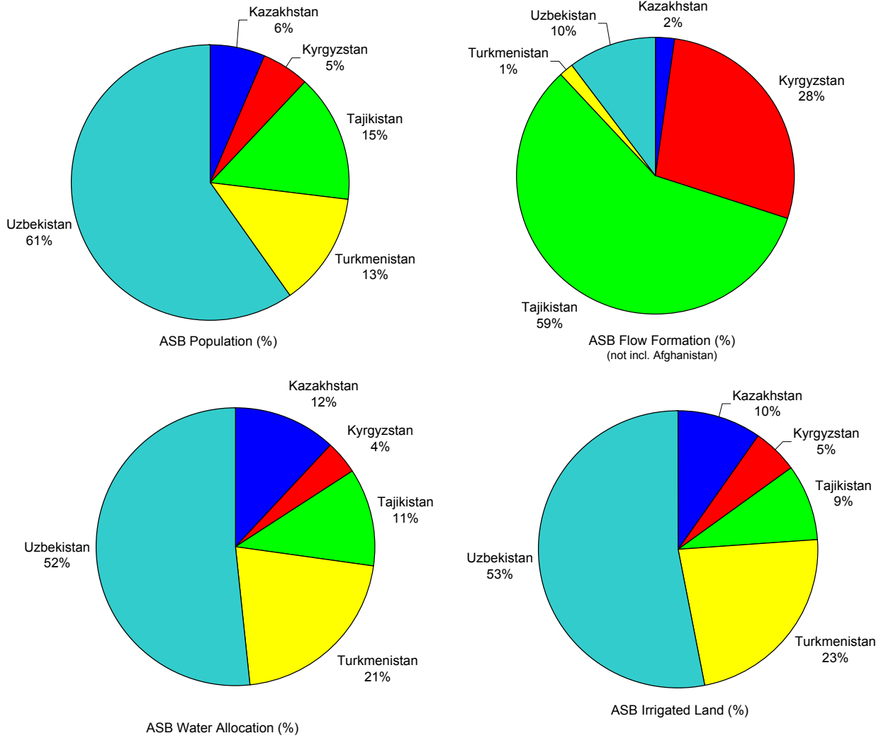
Figure 2. Aral Sea Basin Selected Characteristics: (a) Population; (b) Surface Water Flow Formation; (c) ICWC Water Allocation; and (d) Irrigated Lands.
