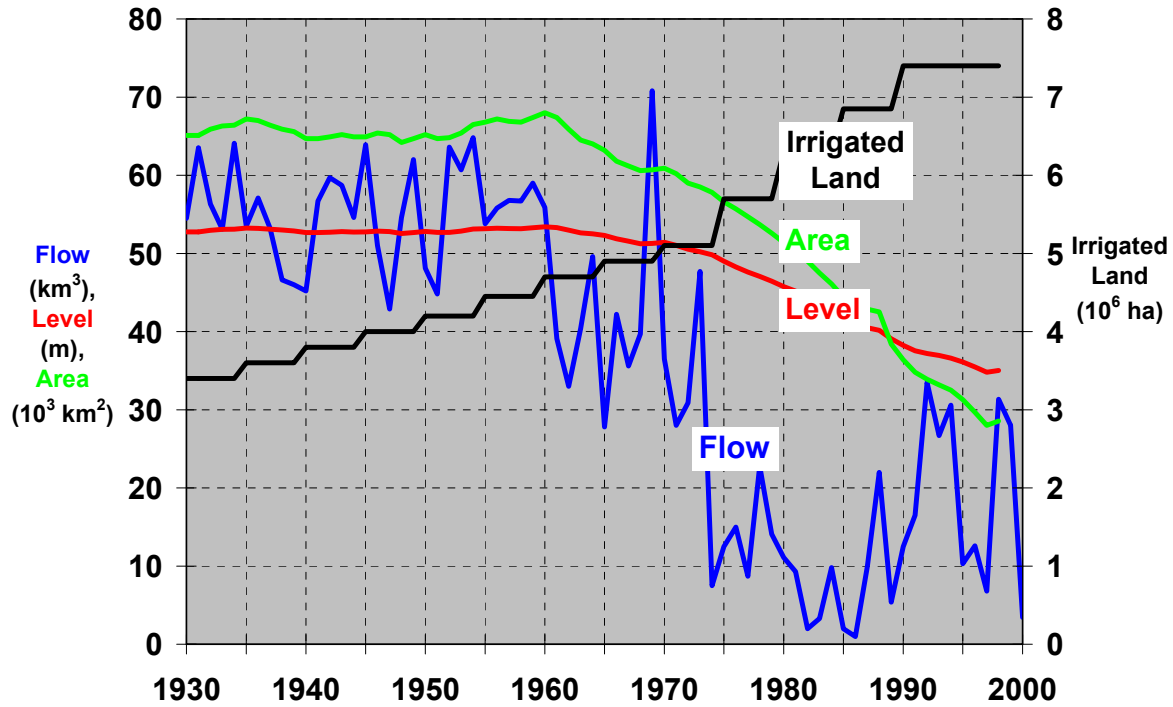
Figure 3. Decline of the Aral Sea with Increased Irrigated Area in Central Asia
