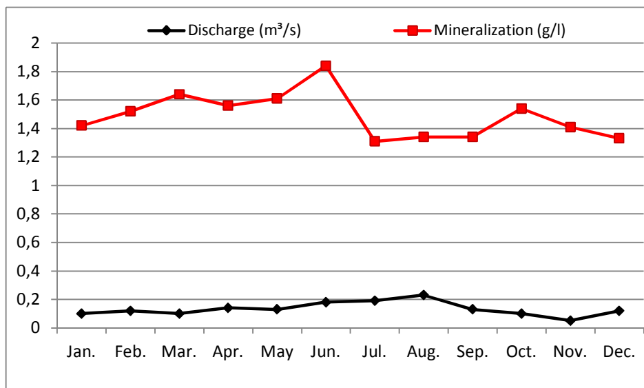
Fig. 12: Discharge (m³/s) and mineralization (g/l) of the collector Cheganak in 2003
