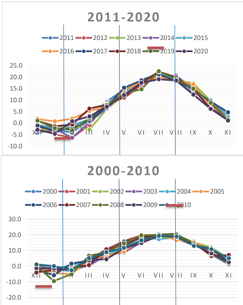
Fig. 4. Temperature changes in the Kashkadarya River basin measured by the traditional method.
