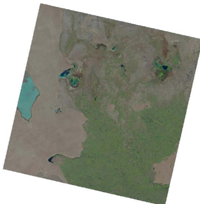
Figure 2 The Aral Region. Landsat 8, 03 October 2021. Clouds 0%
