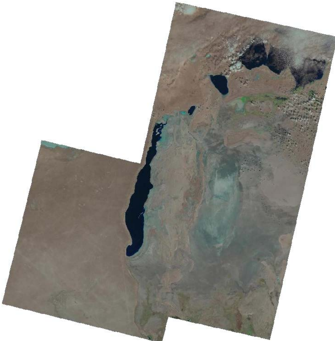
Figure 1. Western and Eastern parts of the Aral Sea. Landsat 8, 03 October 2021. (Cloud coverage less than 27 % in the study zone)
