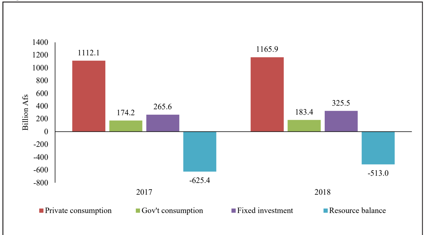
Graph 7-4: Structure of Demand
